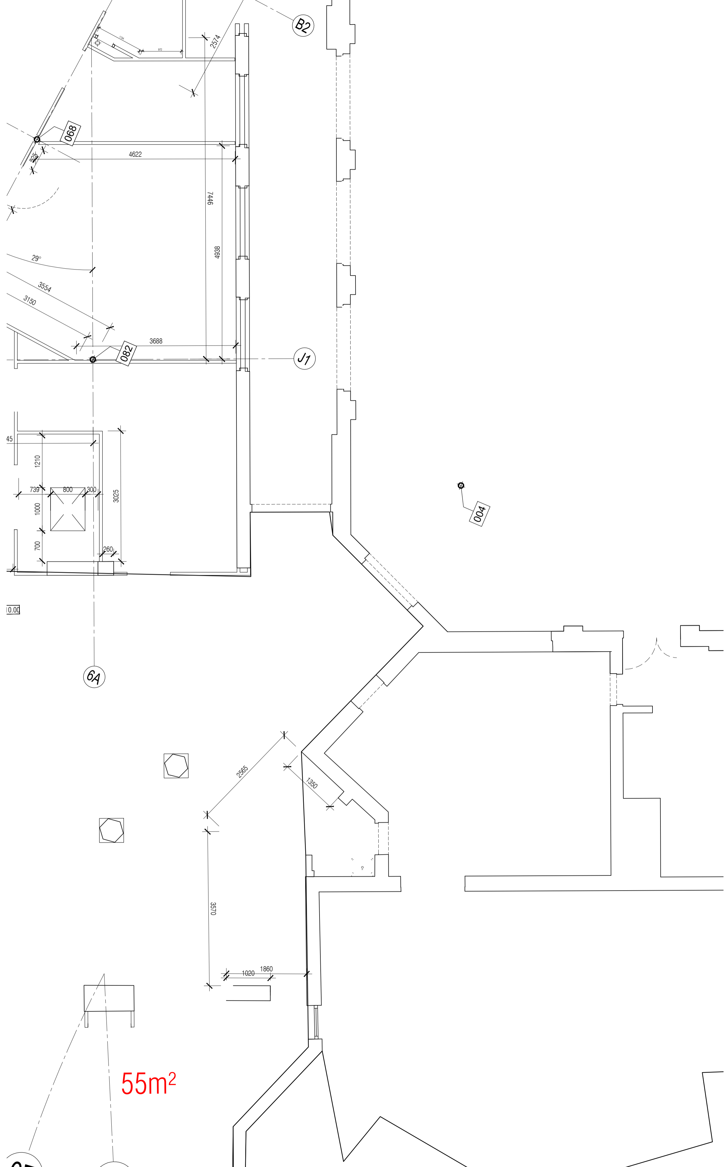
02 Ground Floor Coordinates Plan Scale: 1:50
