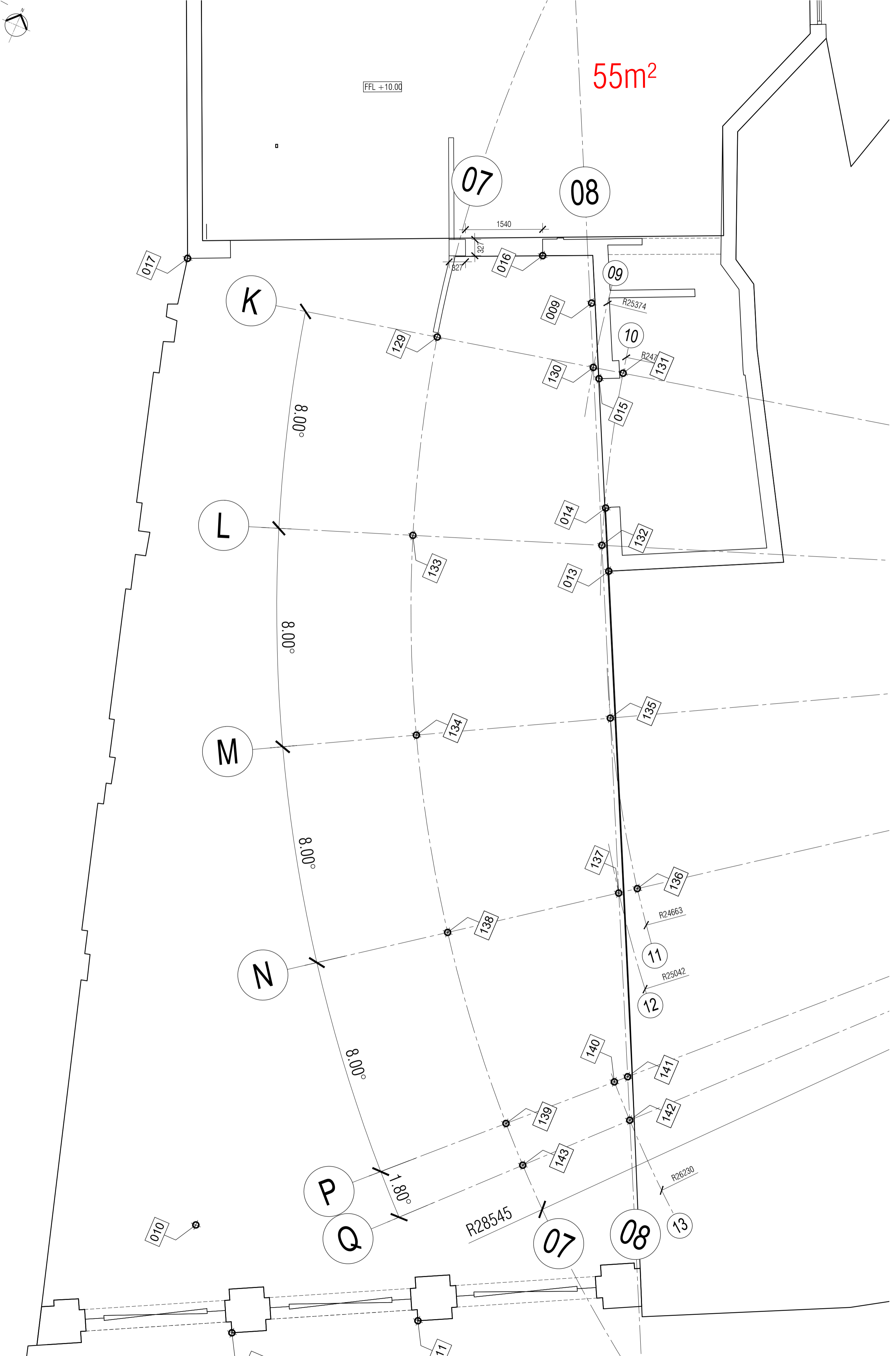
01 Ground Floor Coordinates Plan Scale: 1:50
