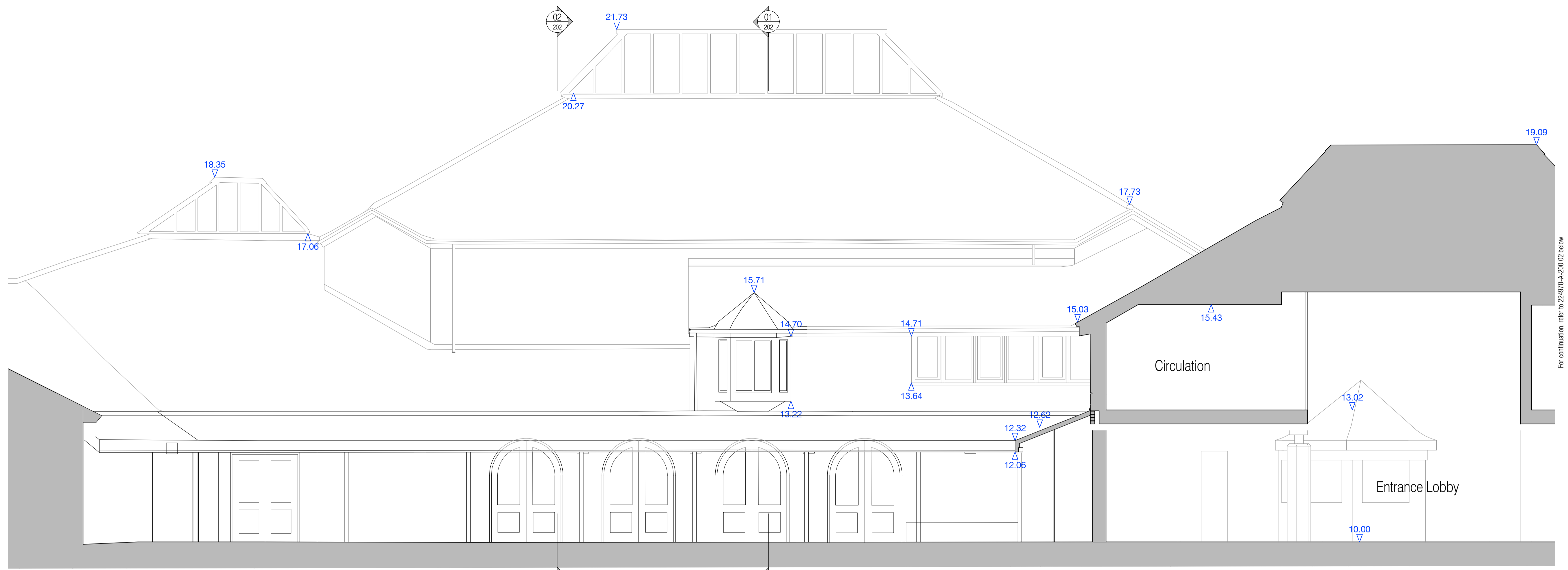
01 Section 02 North Scale:1:50
