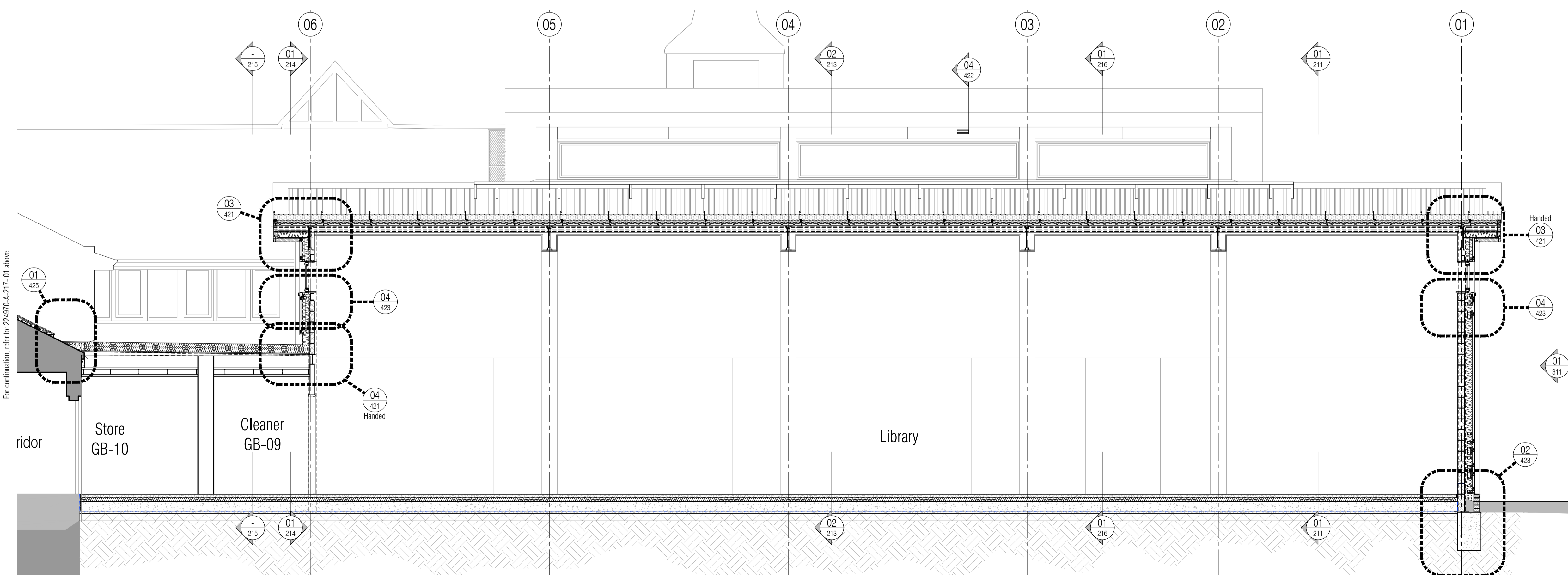
02 Section 06 West Scale:1:50
