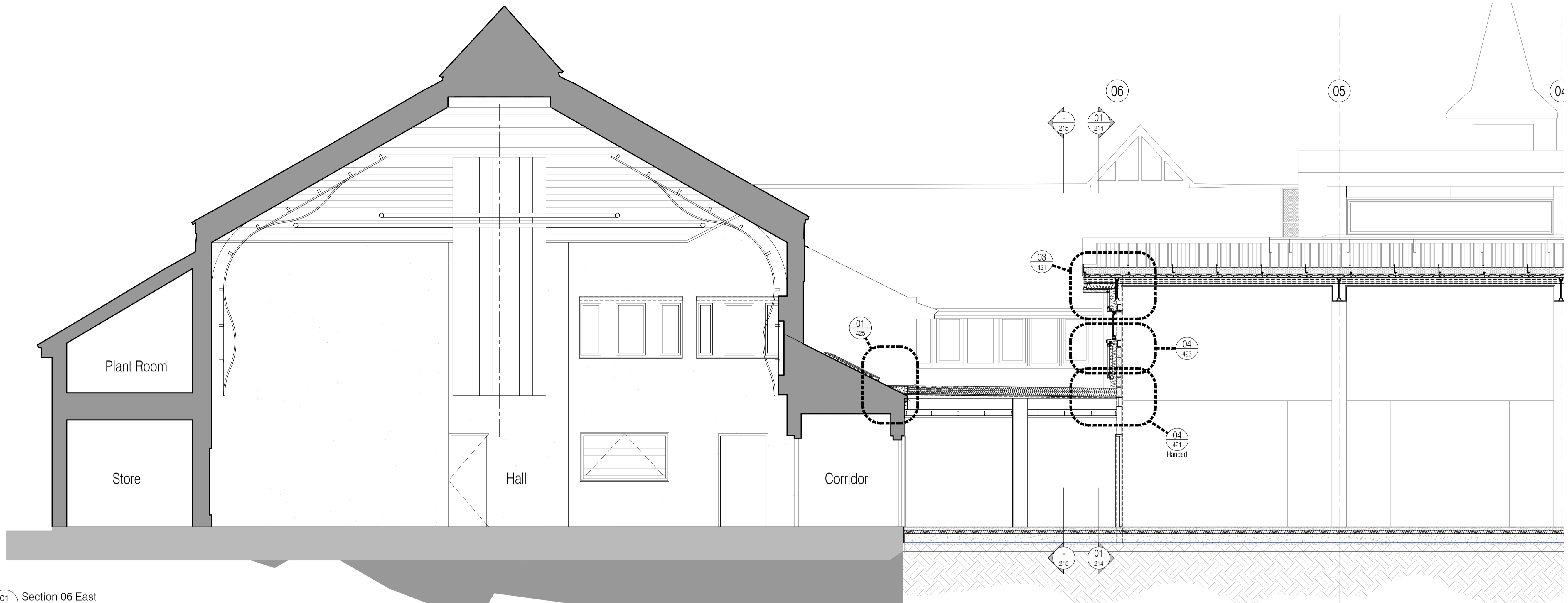
01 Section 06 East Scale:1:50
