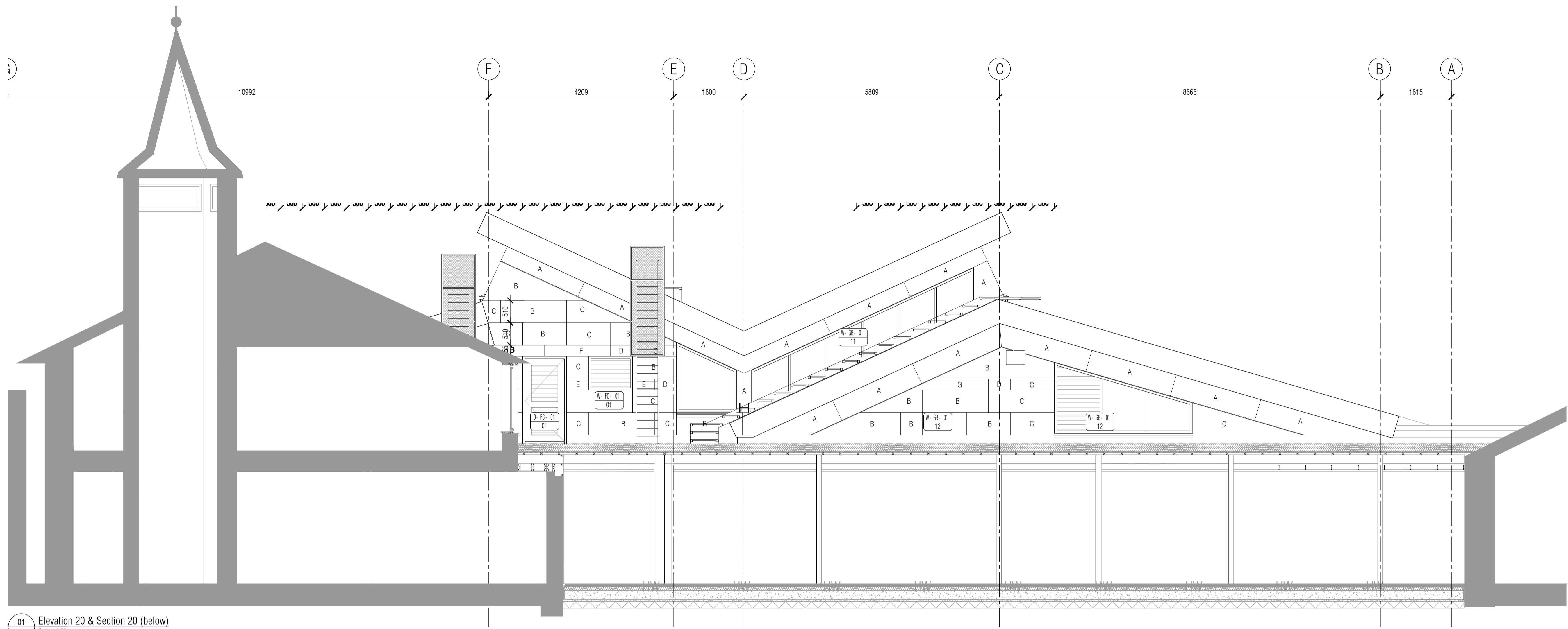
01 Elevation 20 & Section 20 (below) Scale: 1:50
