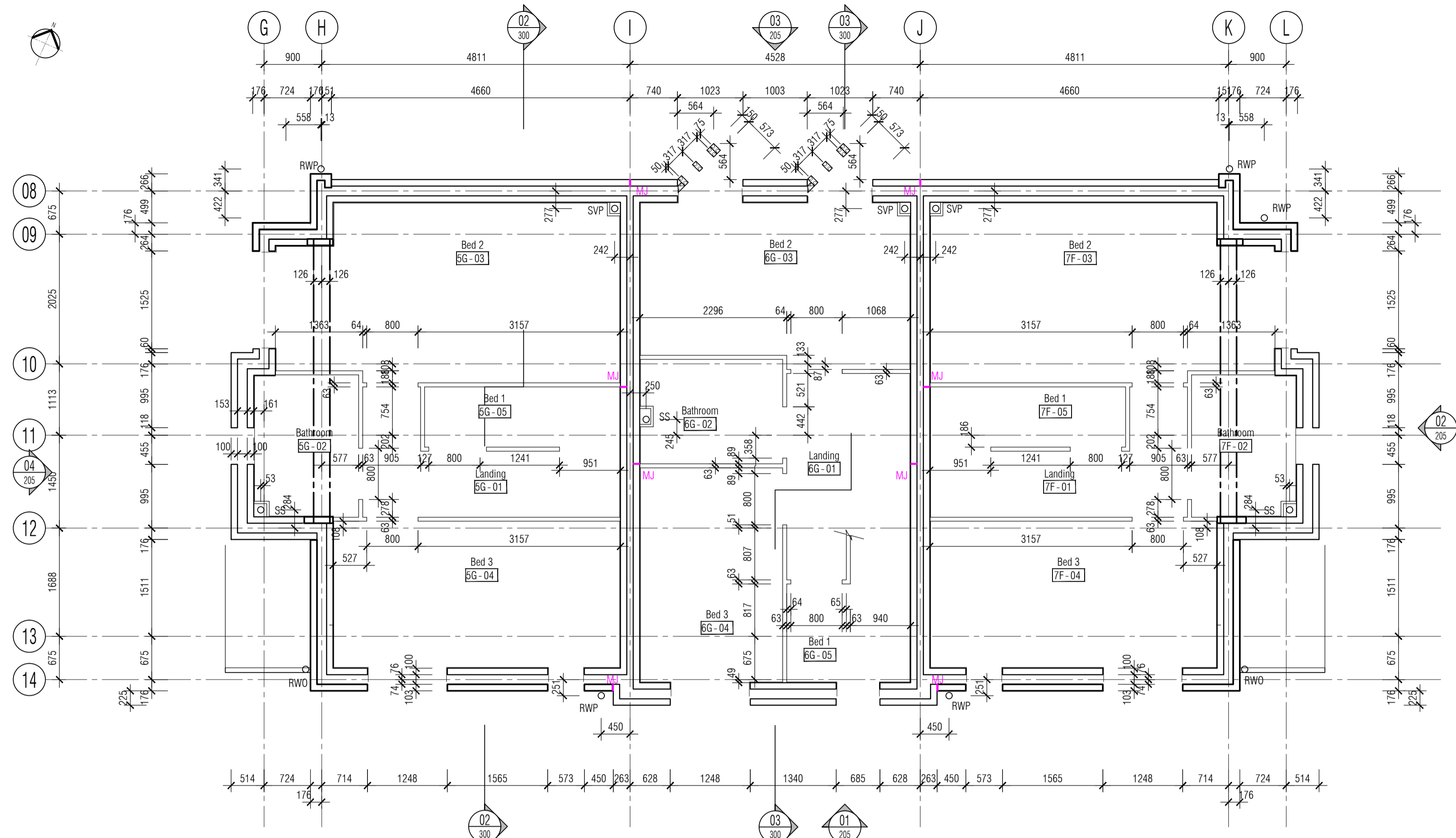
01 Proposed First Floor Setting Out Plan Scale: 1:50
