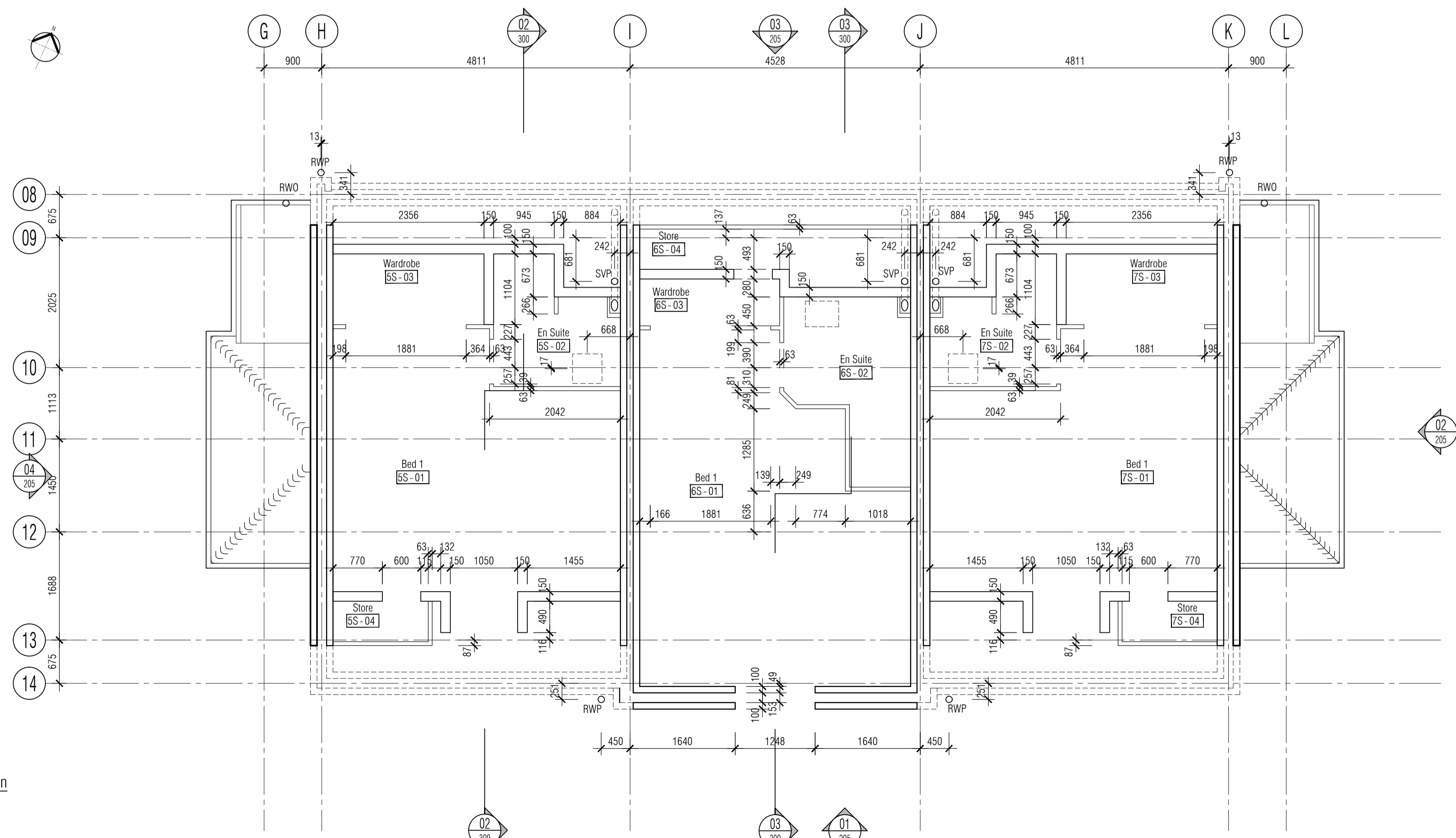
02 Proposed Second Floor Setting Out Plan Scale: 1:50
