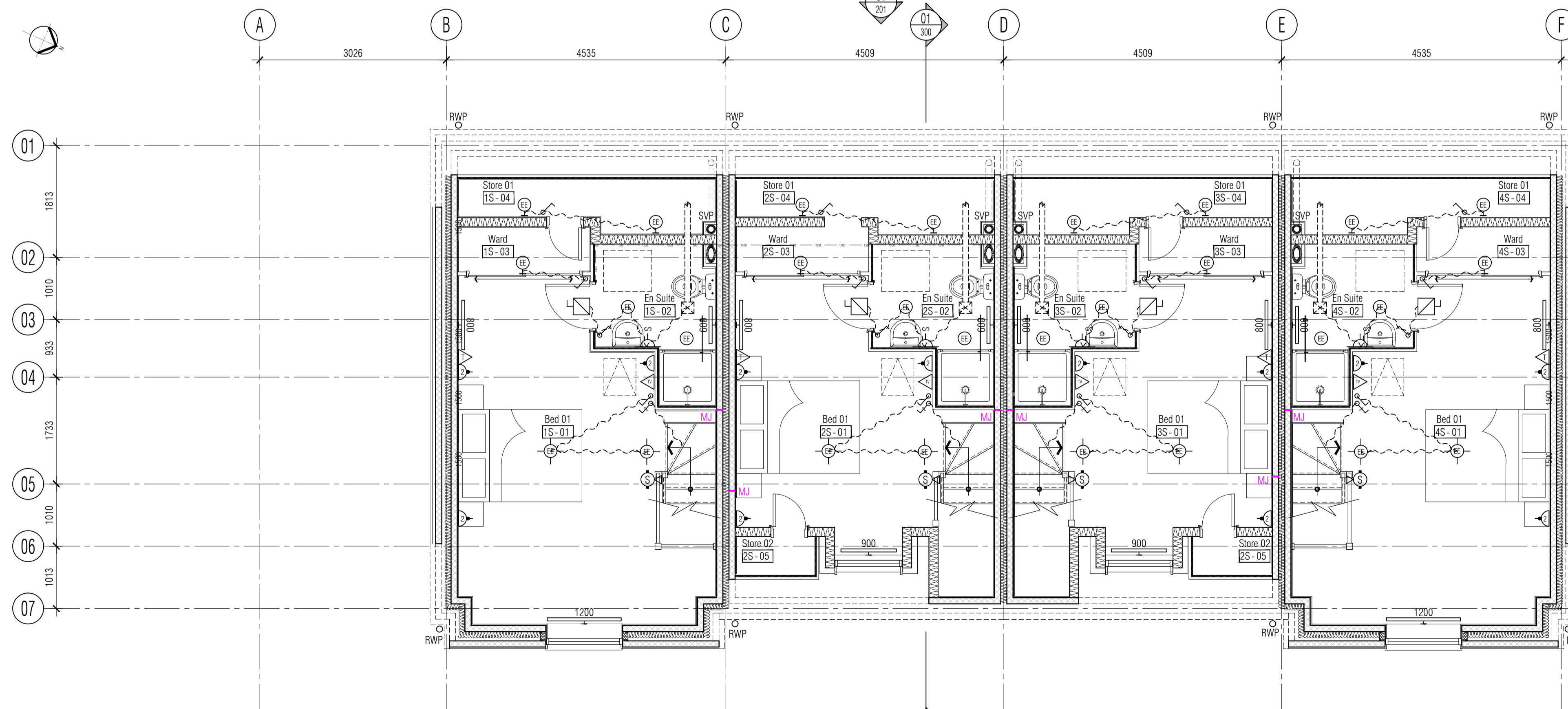
02 Proposed Second Floor Services Plan Scale: 1:50
