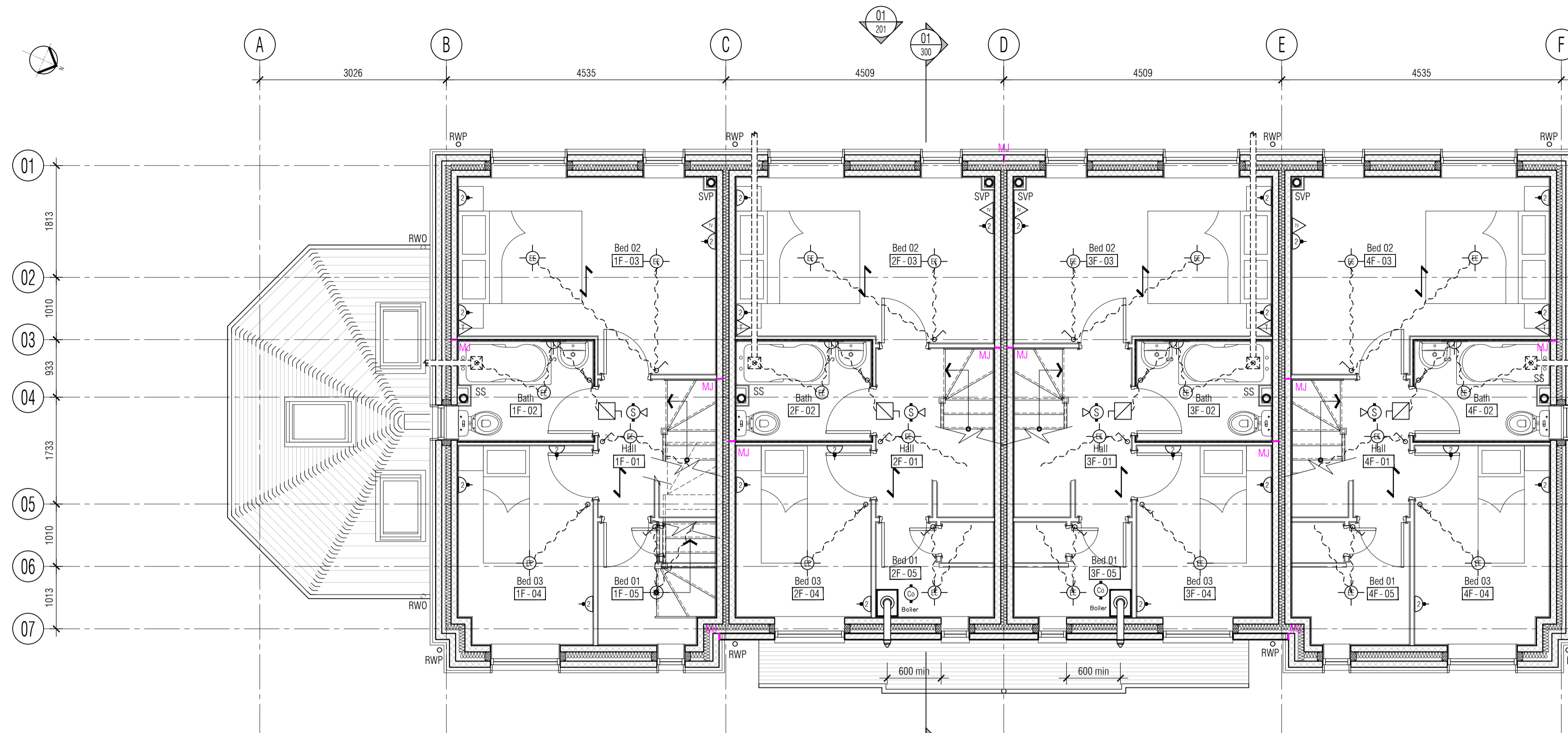
01 Proposed First floor Services Plan Scale: 1:50
