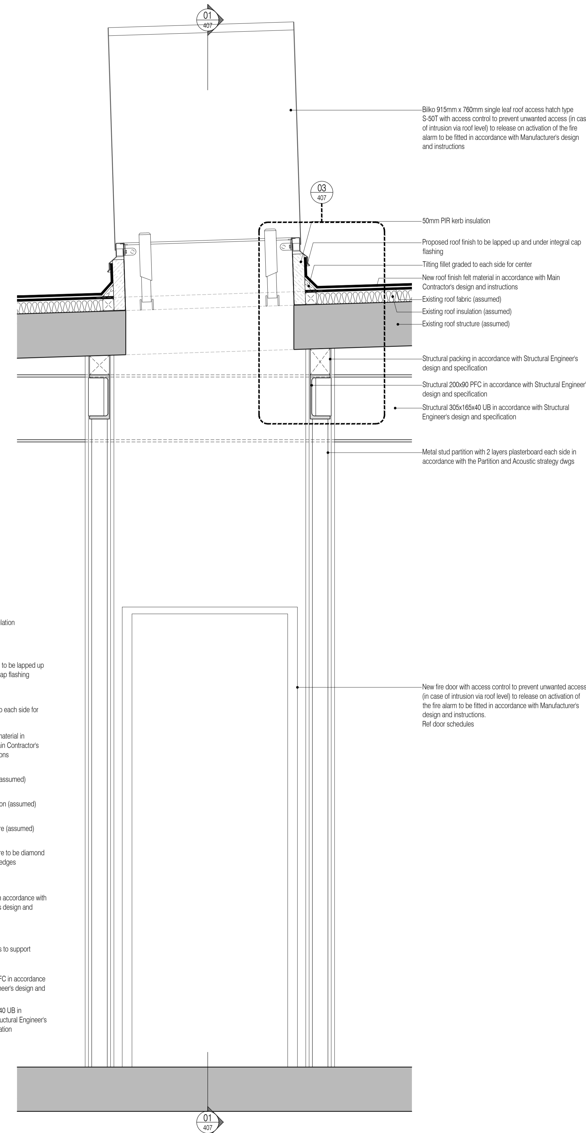
02 Section 09 thro' Roof Hatch Scale: 1:10
