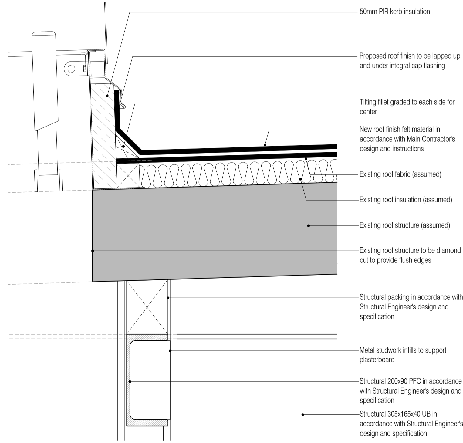
03 Roof Hatch Kerb Detail Scale: 1:10
