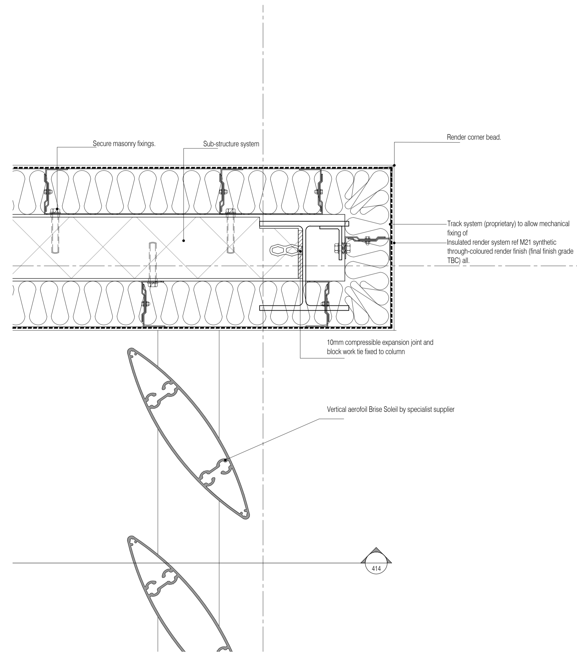
03 Plan Scale:1:10
