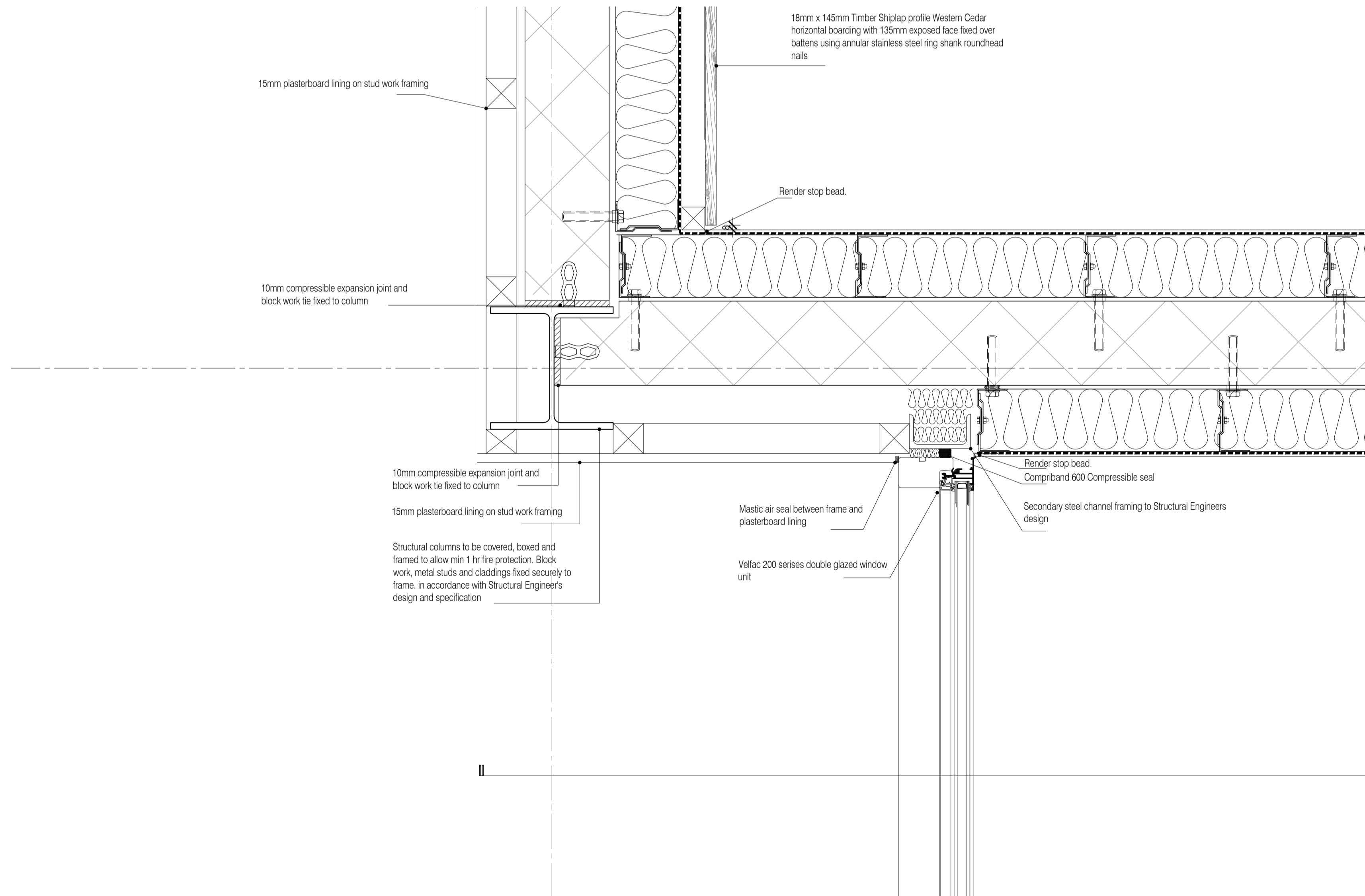
02 Plan Scale:1:10
