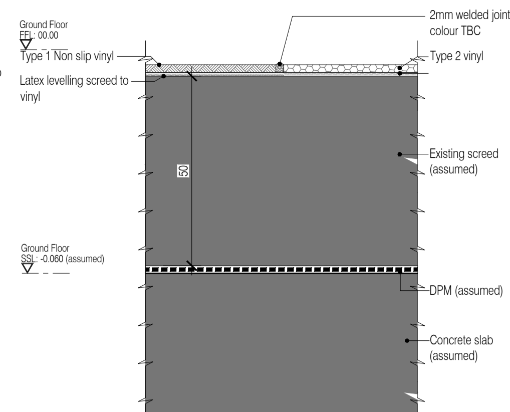
17 Non-slip Vinyl Type 2 / Vinyl Type 2 Interface Scale:1:1
