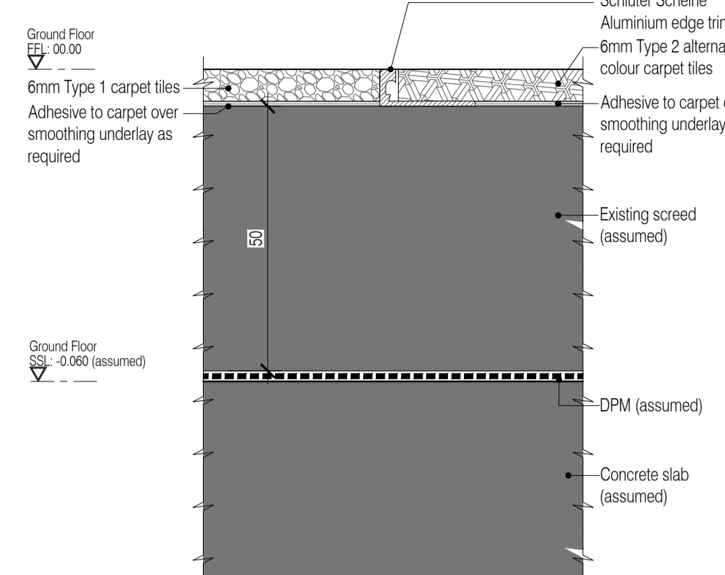
19 Carpet tiles Type 1 / Circulation & Stair Carpet Interface Scale:1:1
