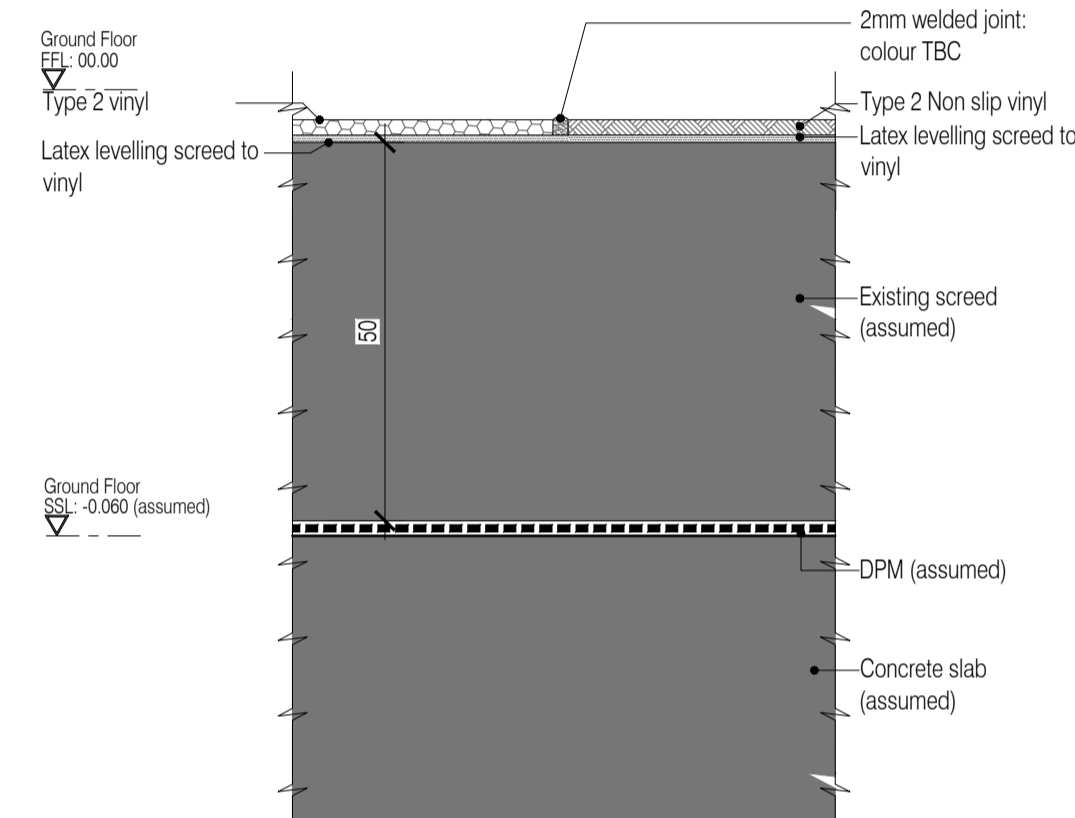
21 Vinyl Type 2 / Non slip vinyl Type 2 Interface Scale:1:1
