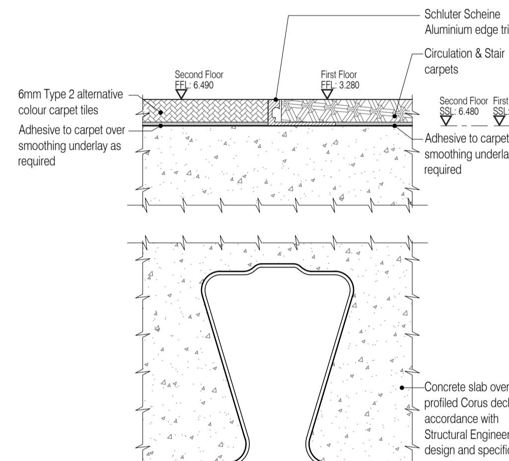
24 Carpet tiles Type 2 / Circulation & Stair carpet Interface Scale:1:1
