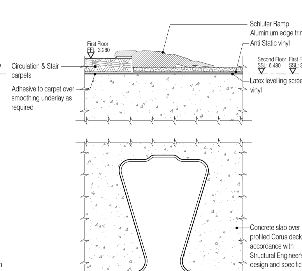
25 Circulation & Stair carpet / Anti Static Vinyl Interface Scale:1:1
