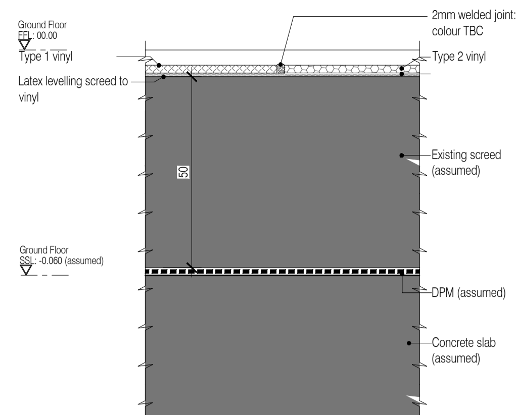
18 Vinyl Type 1 / Vinyl Type 2 Interface Scale:1:1
