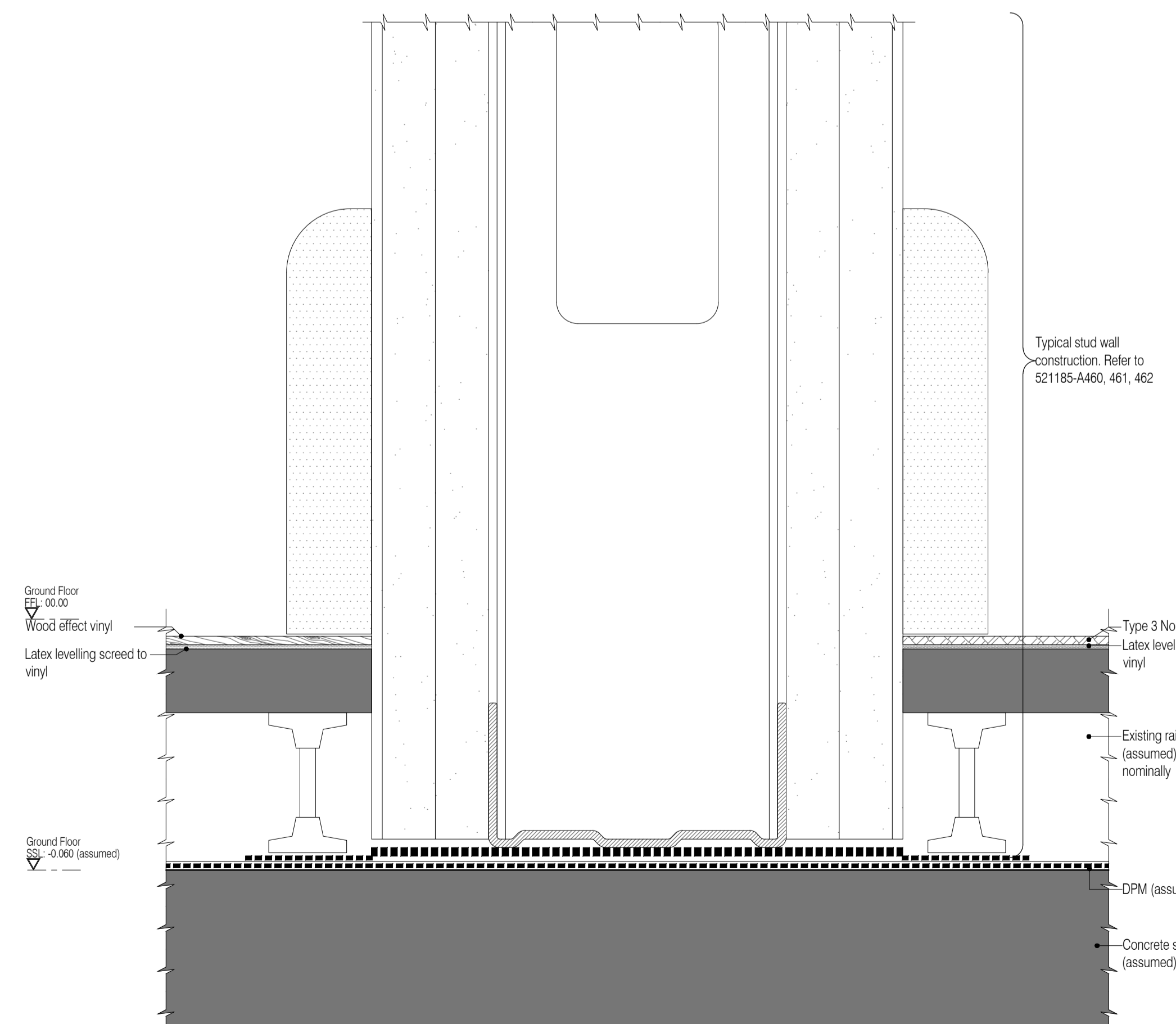
28 Typical Raised Floor Wood effect vinyl / Non slip vinyl Type 3 Interface Scale:1:1
