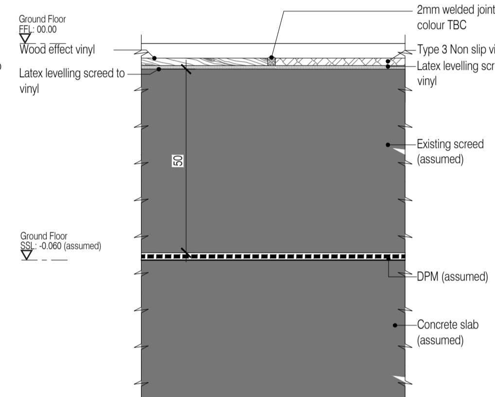
22 Wood effect vinyl / Non slip vinyl Type 3 Interface Scale:1:1
