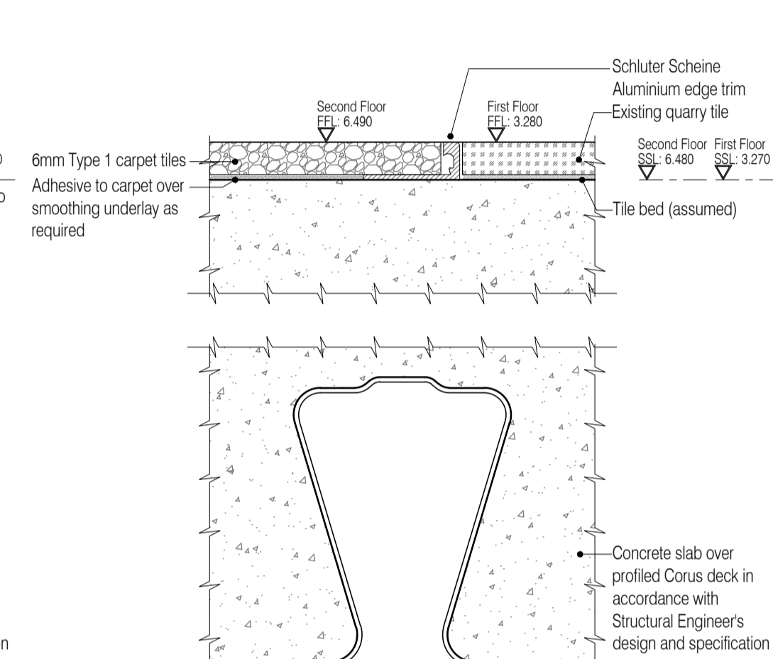
27 Carpet tiles Type 1 / Existing Flooring Interface Scale:1:1
