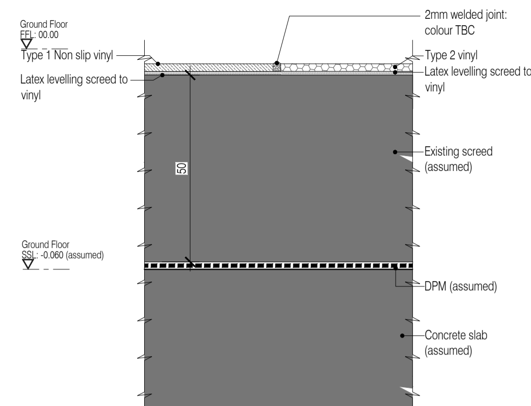
16 Non-slip Vinyl Type 1 / Vinyl Type 2 Interface Scale:1:1
