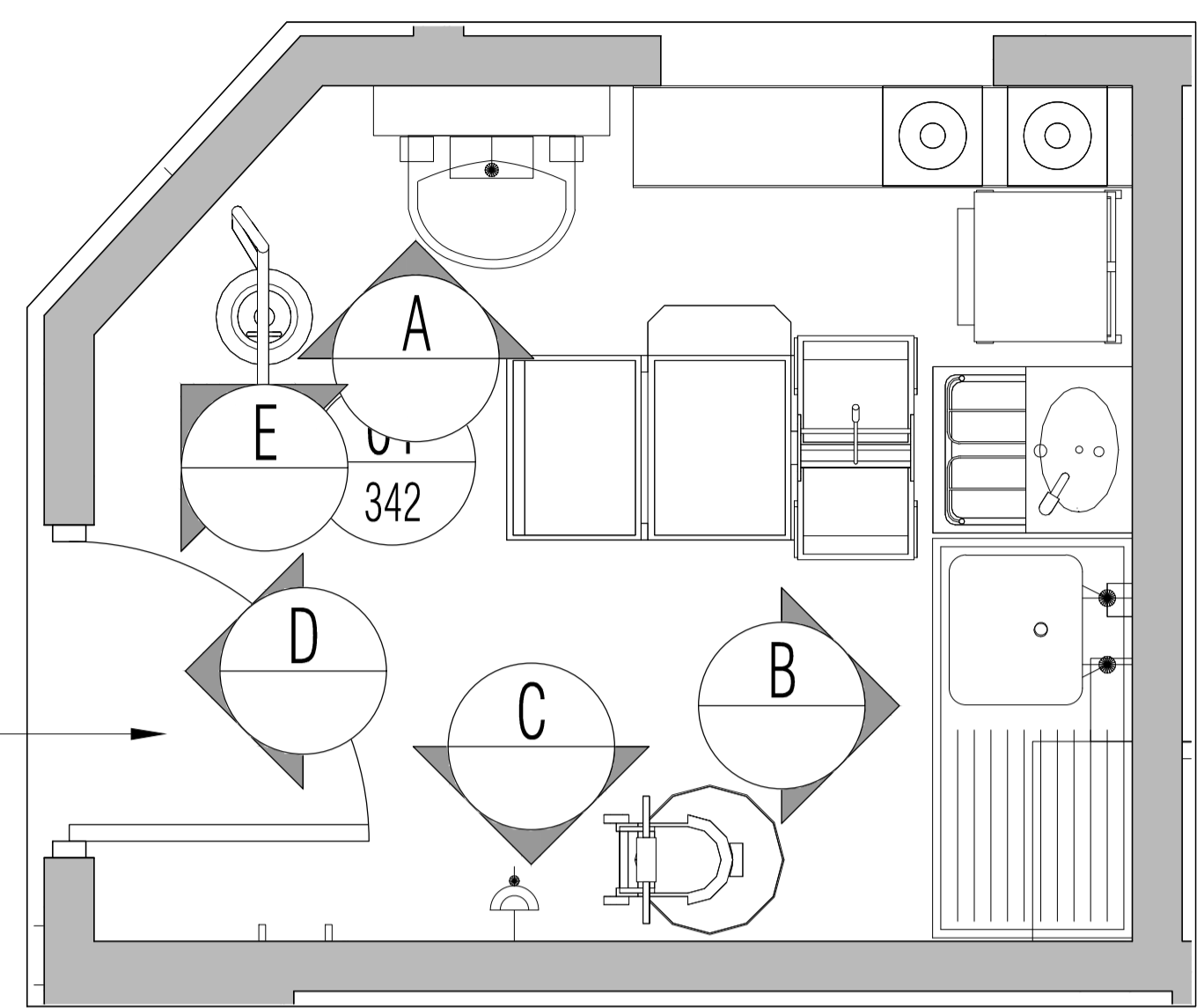
01 1.975 Cleaners Room Scale: 1:20
