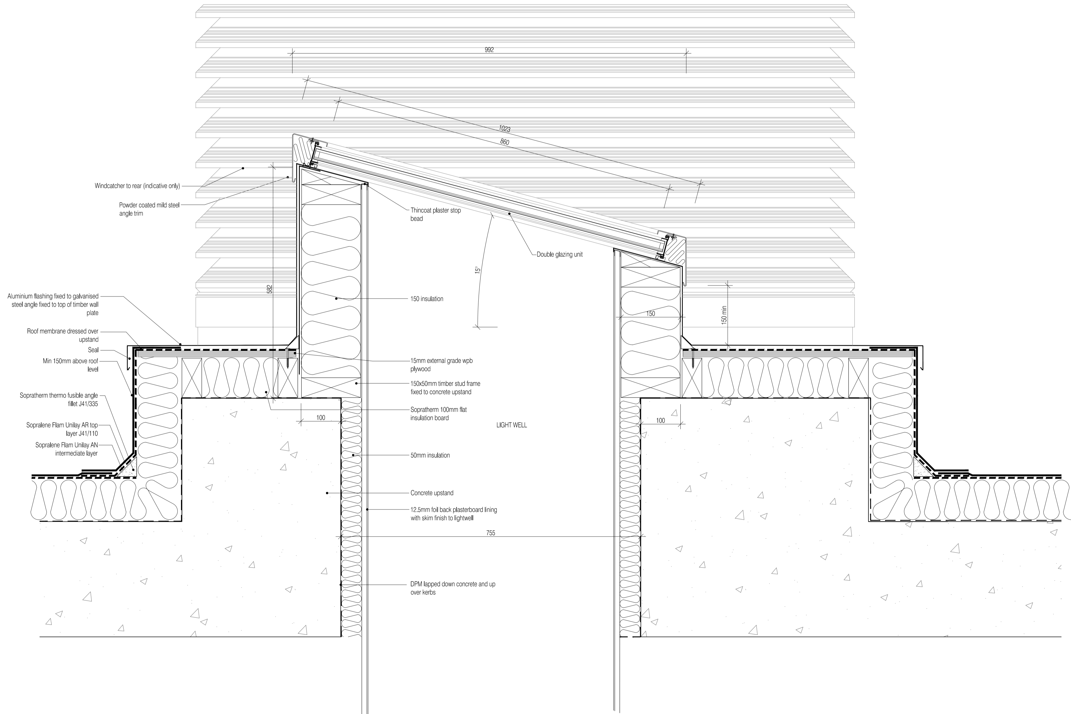
N Section thro' rooflight kerb Scale: ..
