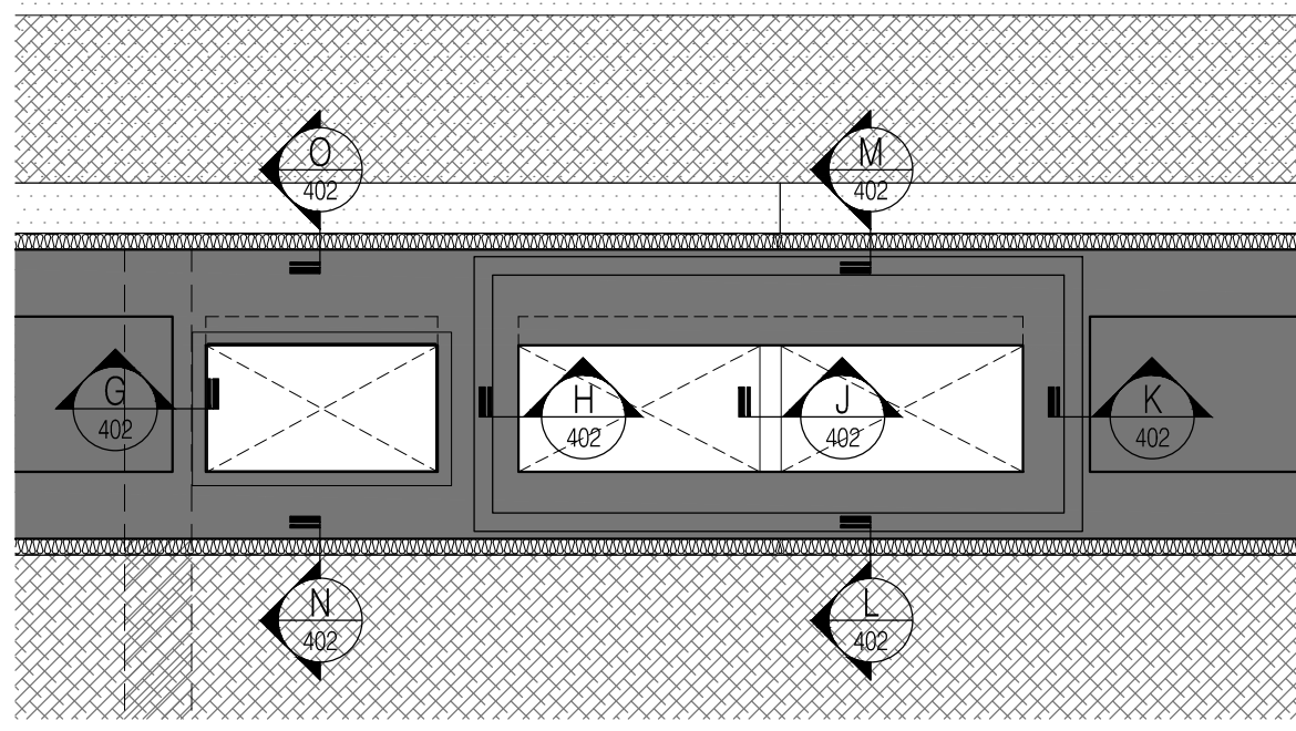
ROOFLIGHT / CHIMNEY KEY PLAN Scale: 1:50
