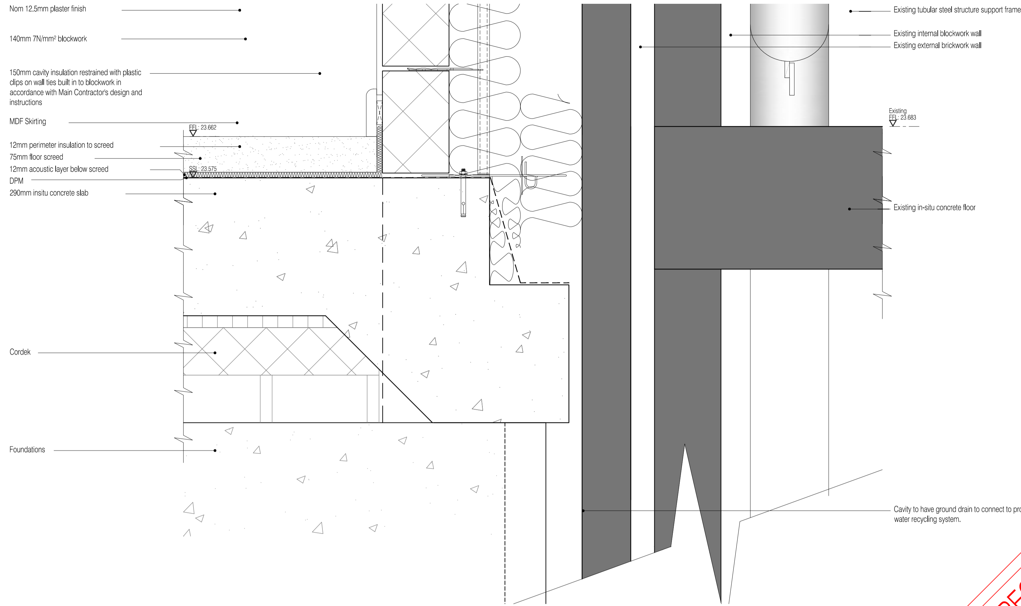
01 Block Y/B Section 1 Ground Channel Detail Scale: 1:5
