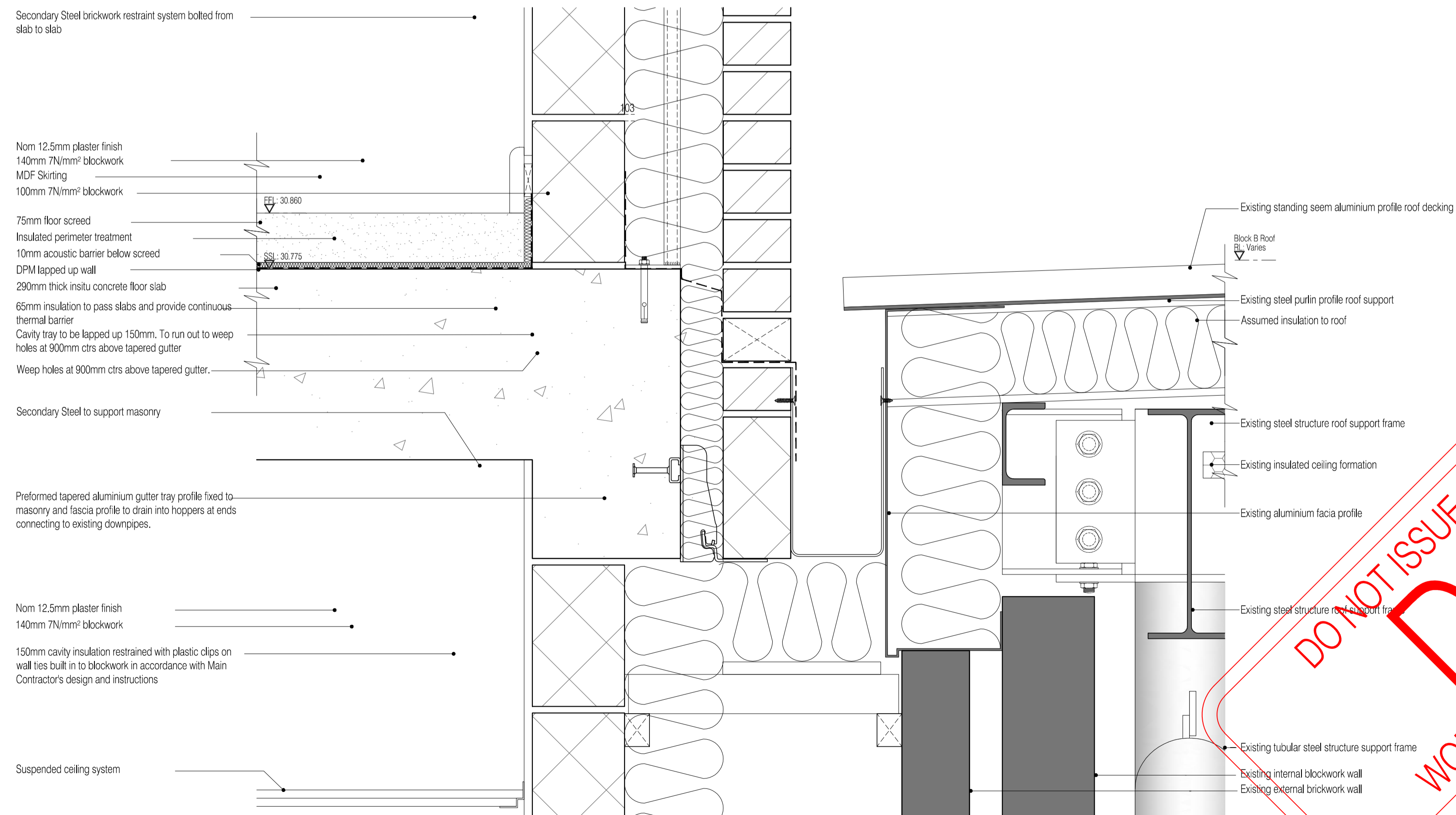
02 Block Y/B Section 3 Gutter Detail Scale: 1:5
