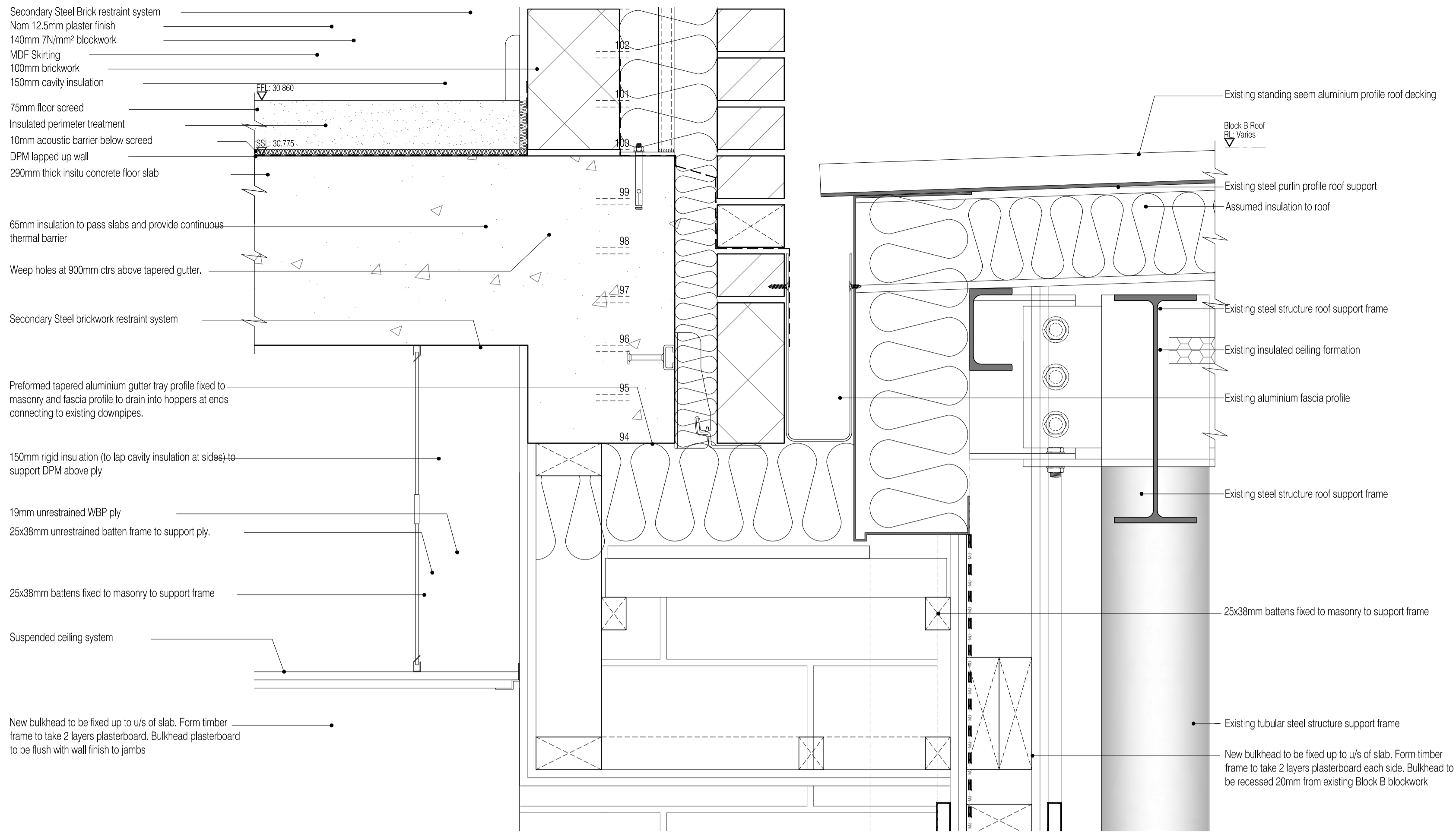
01 Block Y/B Section 1 Gutter Detail Scale: 1:5
