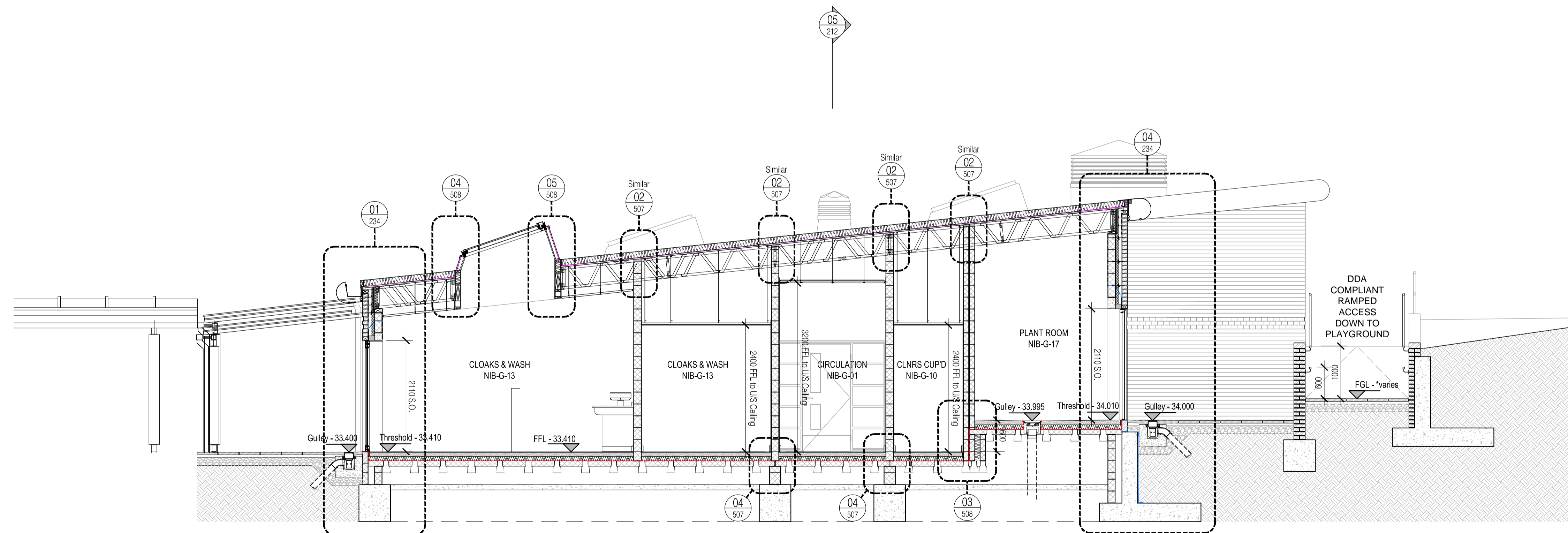
02 Section 2 - Looking North Scale: 1:50
