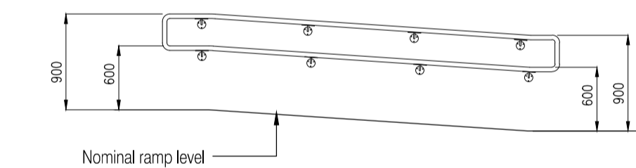
TYPICAL ELEVATION B
