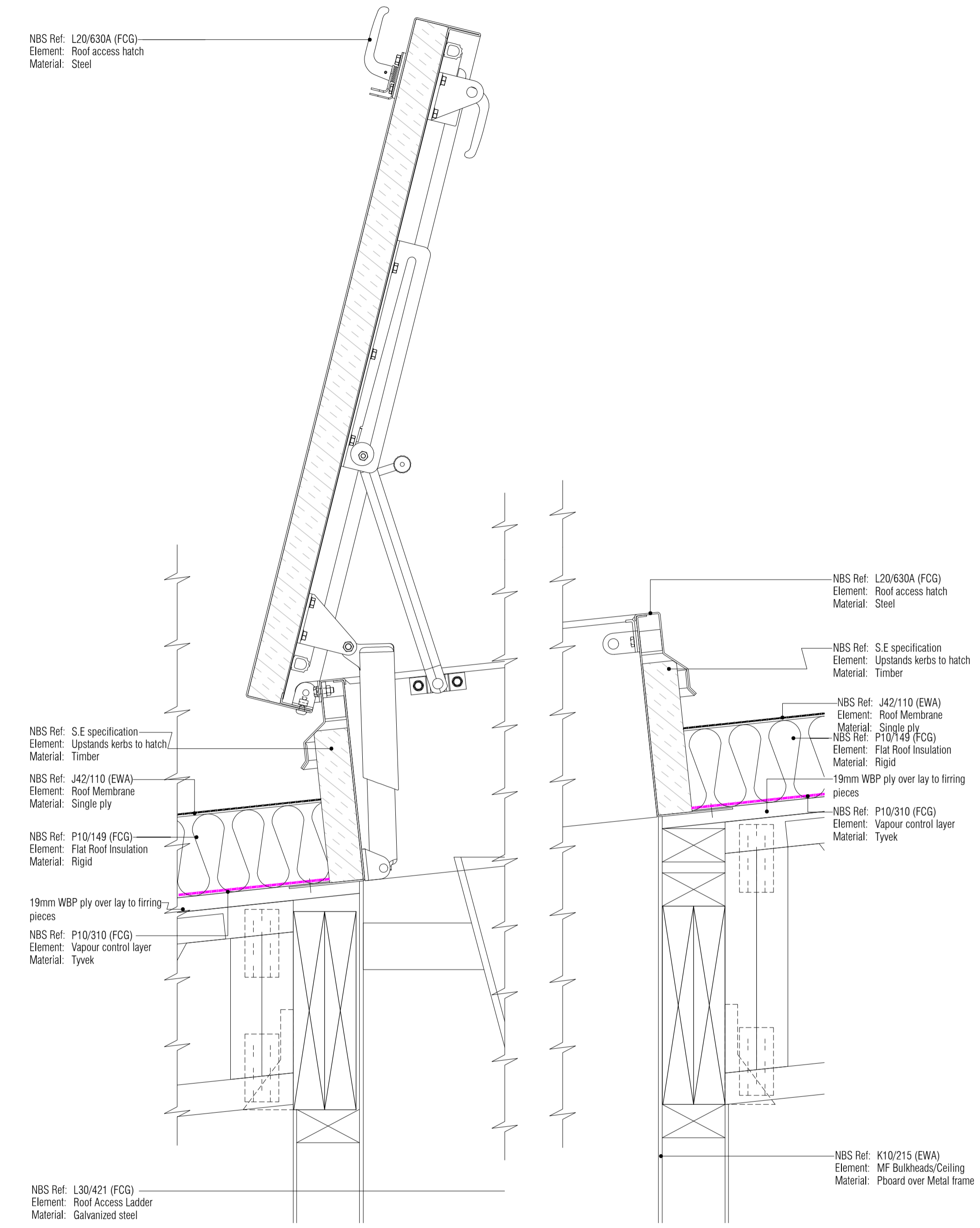
02 Typical Roof Access Hatch Detail Scale: 1:5
